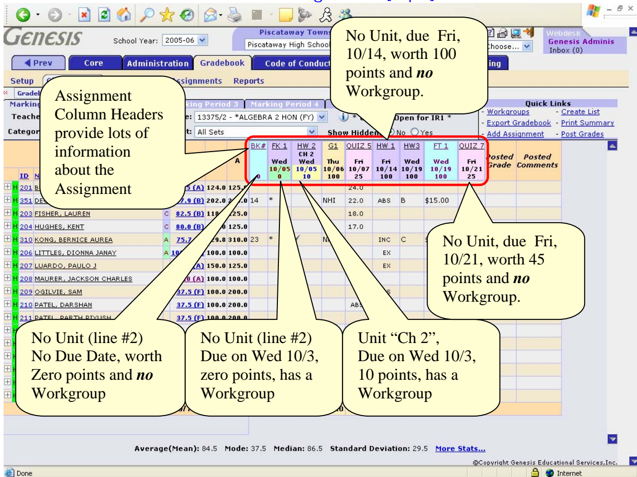
Figure 1 – Gradebook Class Rosters Marking Period Screen
